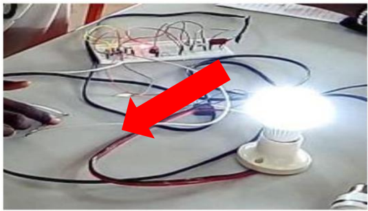
Figure 4: An Automatic light switch on breadboard; (A) Bulb is OFF and (B) Bulb is ON
