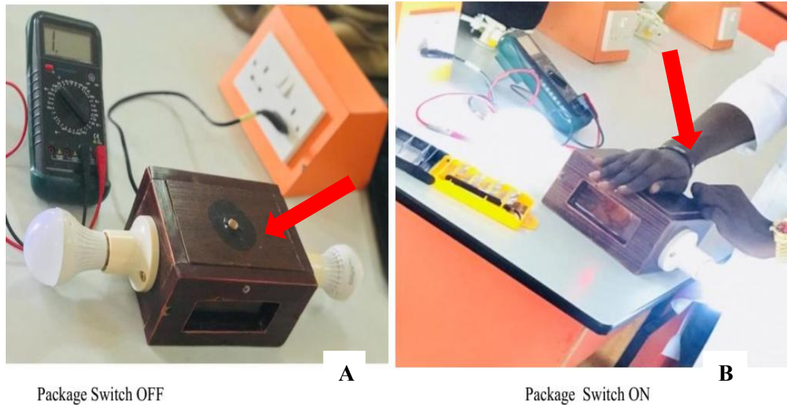
Figure 5: A Prototype A.C automatic light switch package: (A) when Bulb is OFF and (B) when Bulb is ON.
