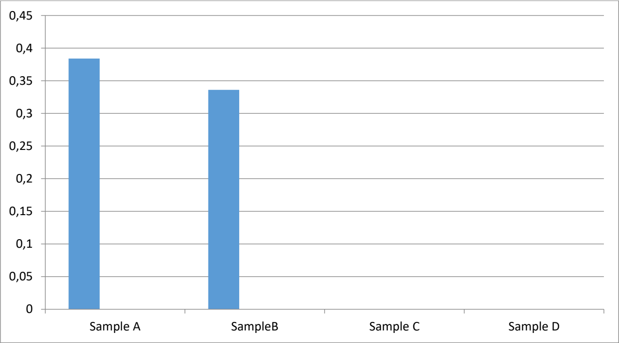
Fig 4: lead concentration
