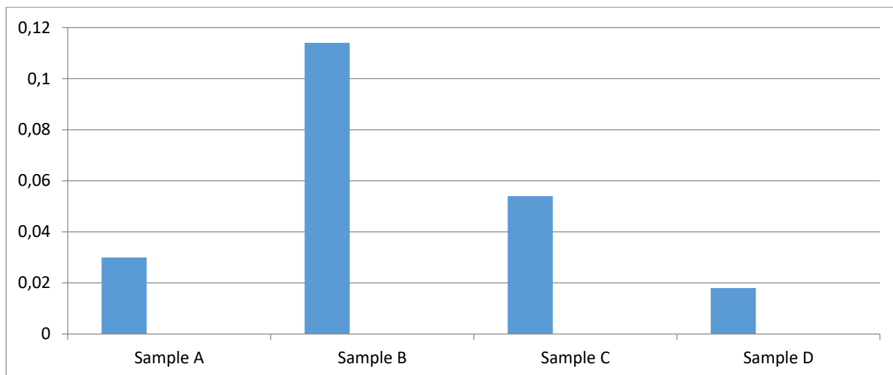
Fig 2.: cadmium concentration
