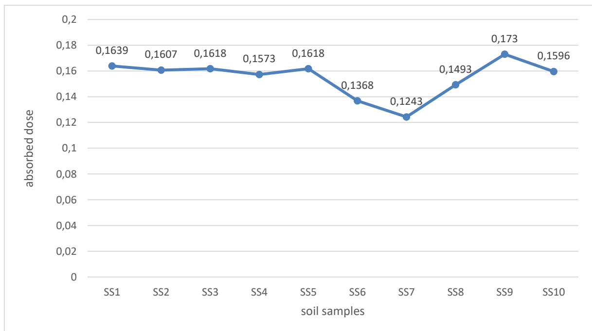
Fig 2: Absorbed dose in Gyhr-1 per soil sample
