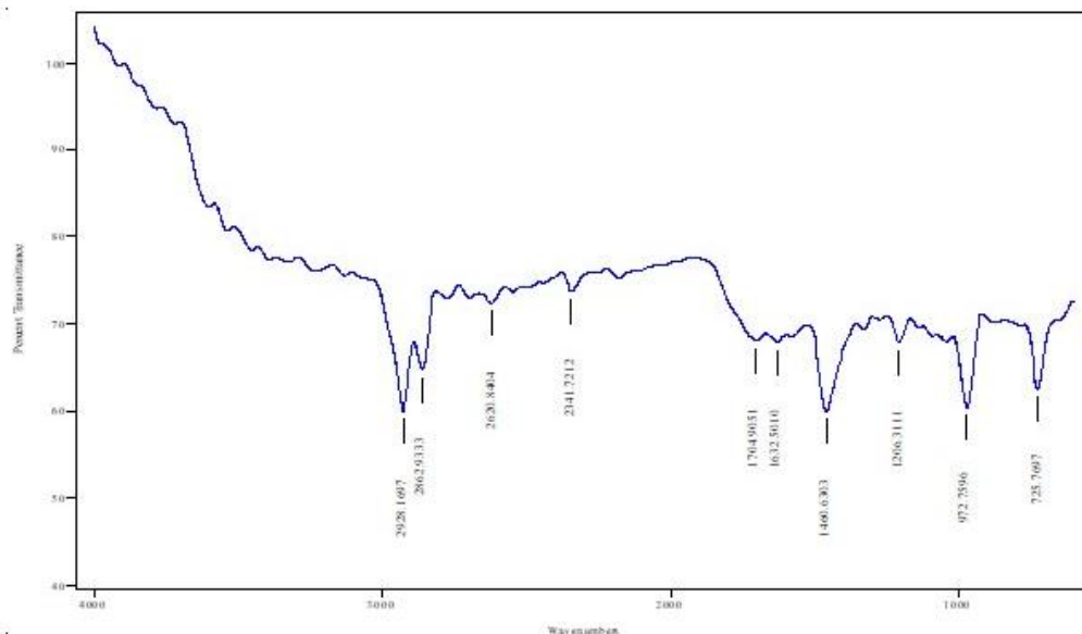
Figure 1: FTIR dye extract from Bridelia ferruginea
