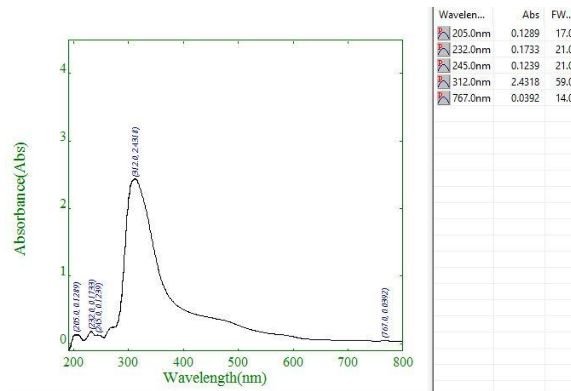
Figure 2: UV-Visible of dye extract from Bridelia ferruginea
