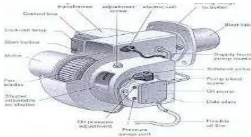
Figure 1: Schematic diagram of the burner (Combustor) Saidur et al, (2011)
