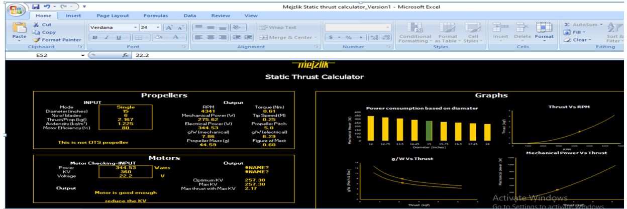
Figure 1.3: Mezjlik Static Thrust Calculator
