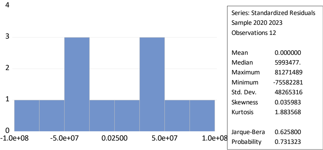
Diagram 1. Standardised Residuals
