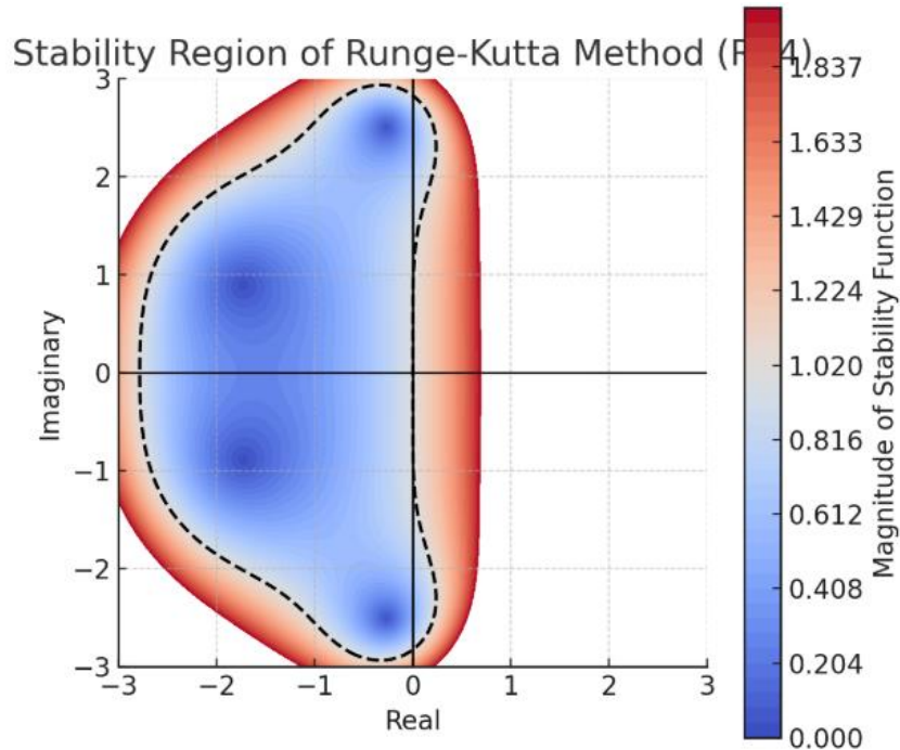
Fig 1: Stability Region of RK4 Method
