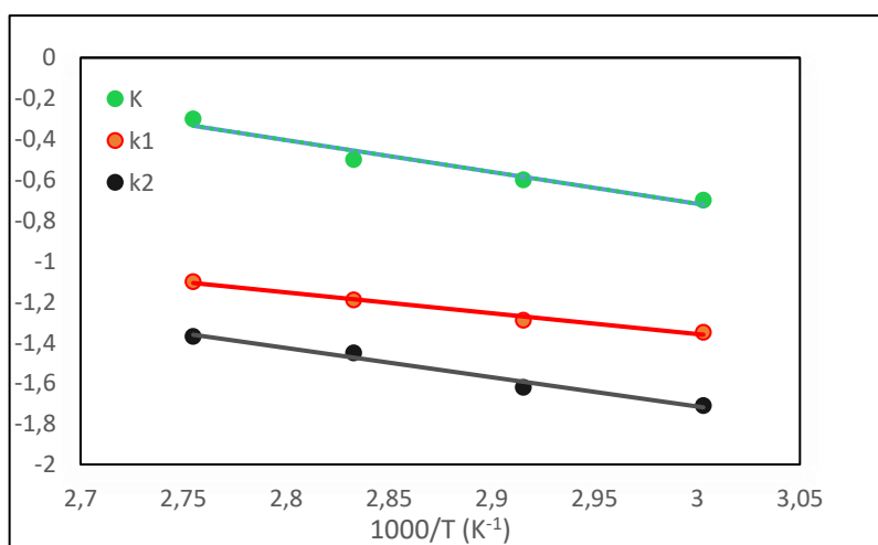
Figure 11: Arrhenius plot of photo oxidation of styrene over \text{Co(0.3)-CeO}_2 catalyst.
