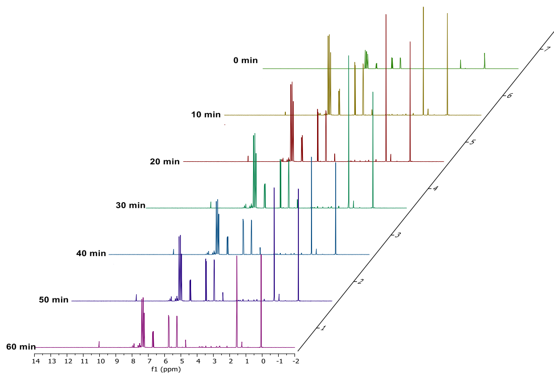
Figure 8: Full spectra of ^1\text{H} NMR of styrene epoxidation after irradiation at 10 min interval for 60 min.
