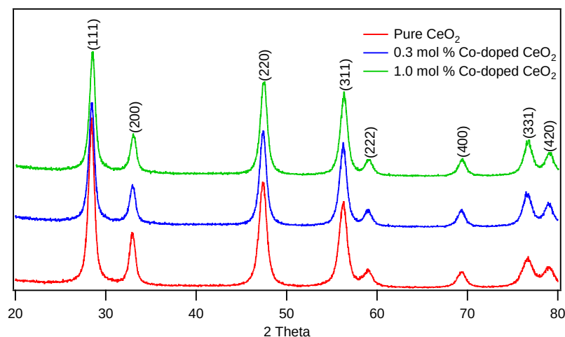
Figure 2: Powder XRD patterns of synthesized pure and cobalt impregnated \text{CeO}_2 NP
