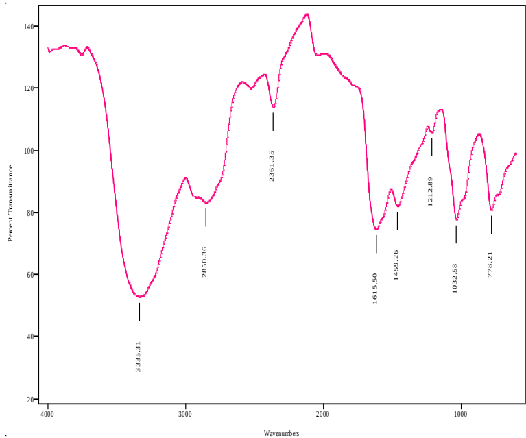
Fig 3 FTIR spectra of beetroot dye extract scanned in the range of 4000cm -1 – 500cm -1 for the functional group of beetroot dye
