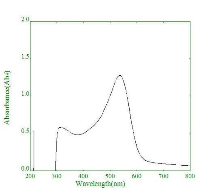
Fig.1 UV- Visible spectra of beetroot dye extract scanned in the range of 200nm-1 –
