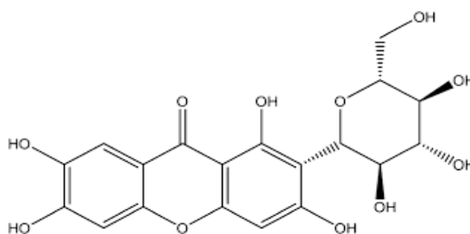
Figure 1: Chemical Structure of Mangiferin
