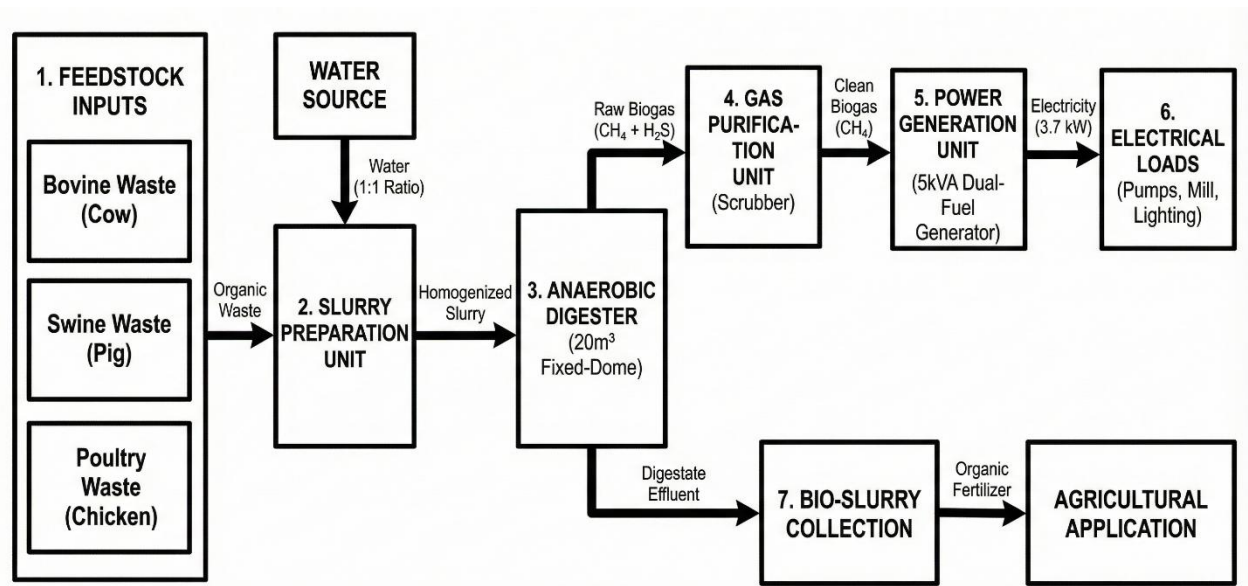
Fig 1: Block Diagram Process Flow of the 3.7 kW Waste-to-Wealth Energy System
