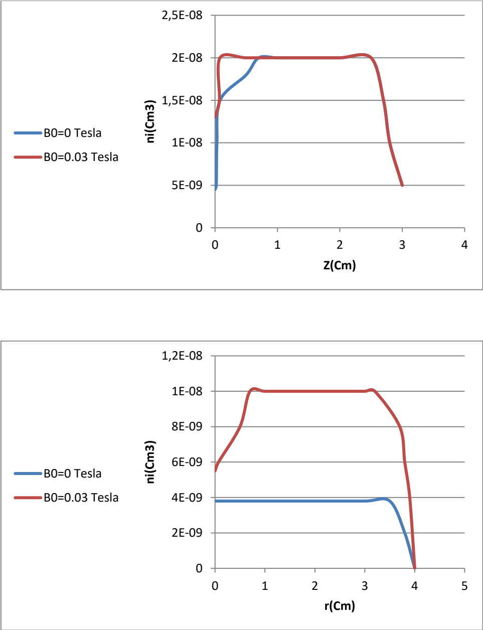
Fig. 4. Position change of ionic density with denotation magnetic field.
