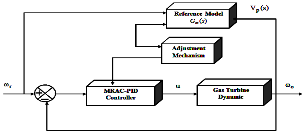
Figure 5: Adaptive-like PID based gas turbine speed control system
