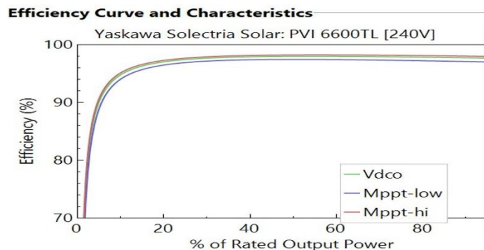
Figure 4: Inverter efficiency curve and characteristic
