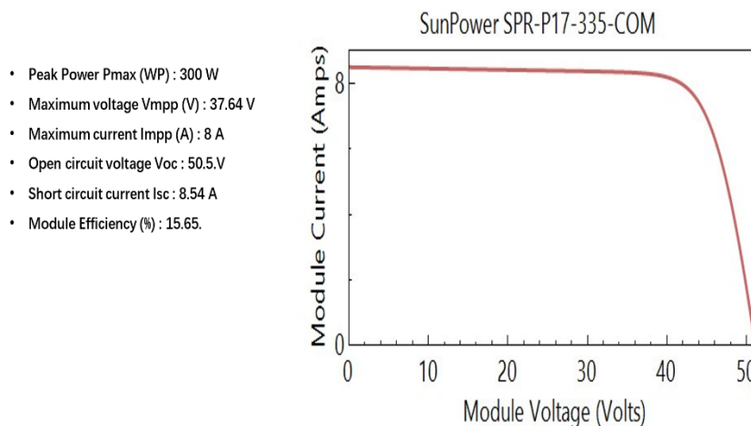
Figure 3: I_V curve(current/voltage)
