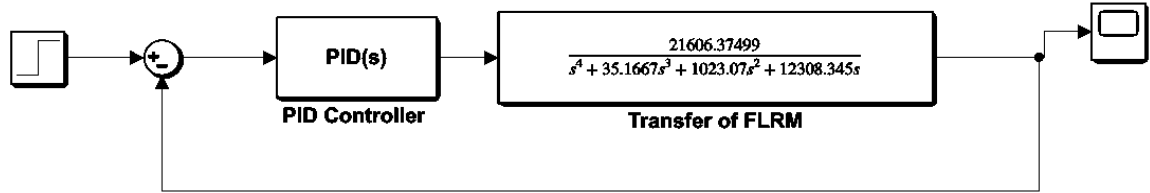
Figure 5: Closed-loop control system with PID in Simulink
