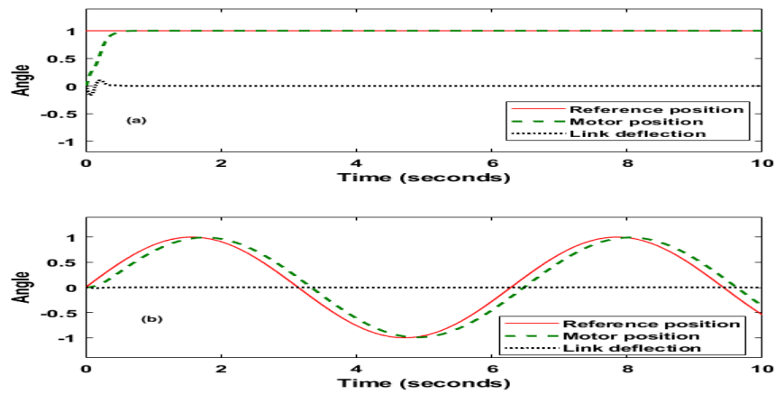
Figure 8: Trajectory tracking of LQR controlled FLRM (a) using step input (b) sinusoidal input
