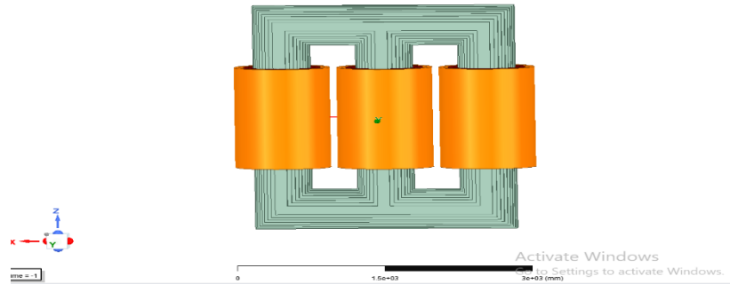
Figure 2: Transformer Model
