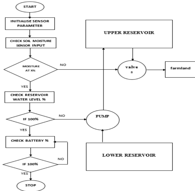
Figure 9 System Flowchart
