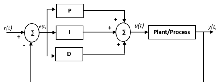
Figure 5: PID Controller
