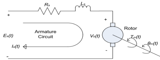
Figure 3: Circuit of a motor (Nise, 2015).
