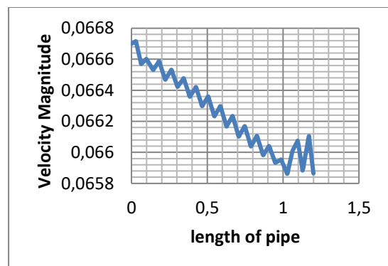
Figure 28: Turbulent flow pattern of water in a pipe along 0.125m at Reynolds number of 10000
