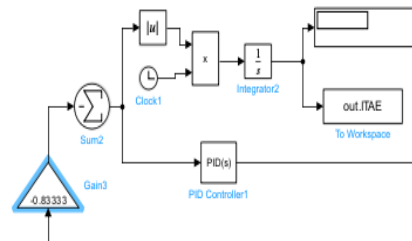
Figure 4: Connecting ITAE to the Output of the PID Controller
