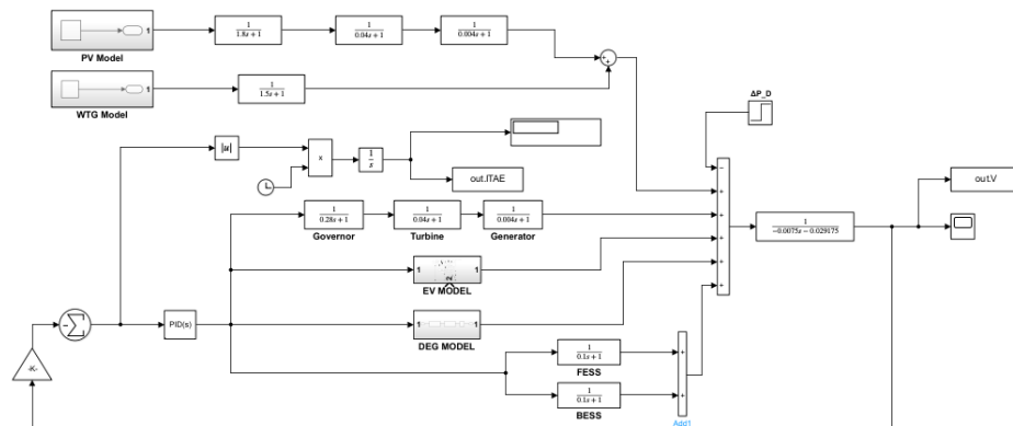
Figure 5: Simulink Model of the Improved SMG System
