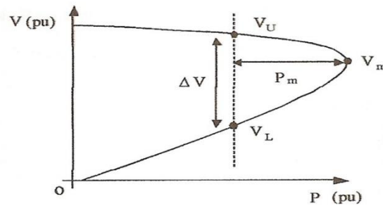
Figure 1: P-V curve [1]
