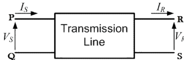
Fig 5 Two port-network
