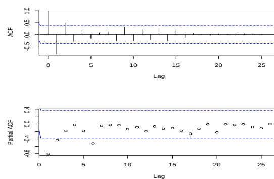
Figure 8. ACF and PACF plot for the second order differenced Alzheimer series.
