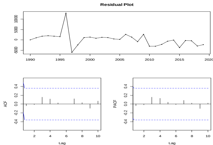
Figure 5: Residual plots for the meningitis series
