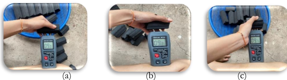
Figure5: Moisture content of the coconut shell, bamboo and mixed briquettes(a,b,c)
