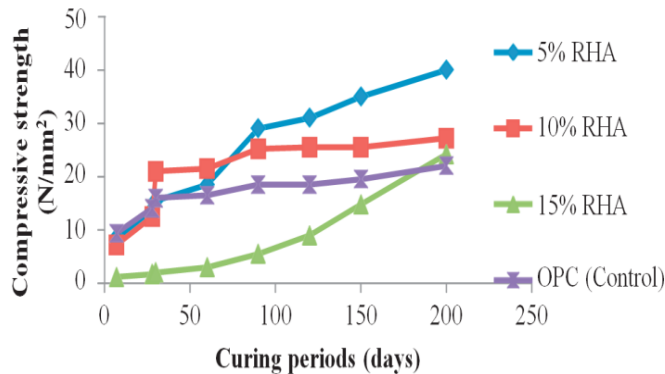
Figure 10 Compressive strength and curing period are corelated at 0%-15% weight of RHA replacement ( Englehardt and Peng , 1995) .
