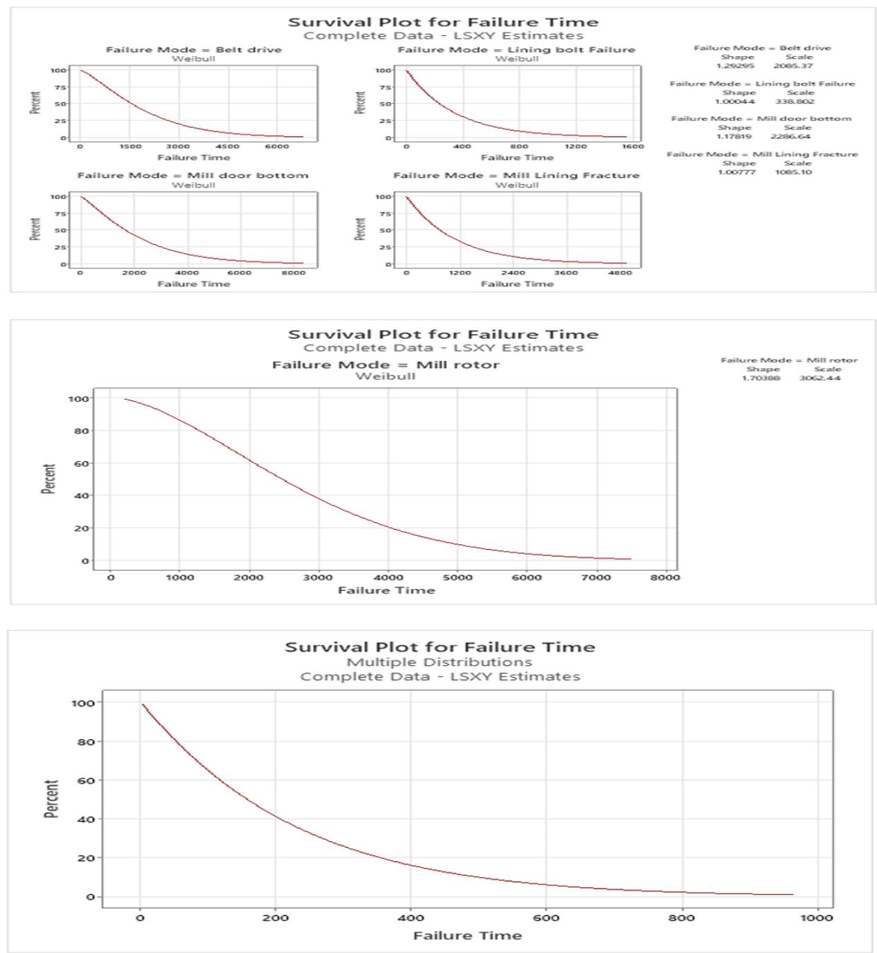
Figure 5. Reliability function curve showing component survival rates
