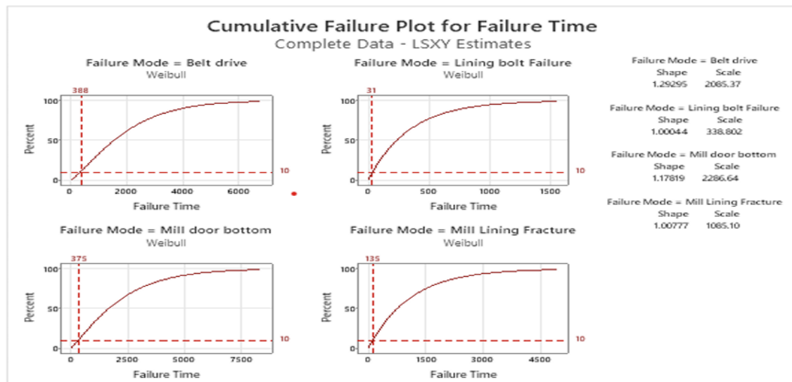
Figure 6. Cumulative Failure plot for Belt drive, Lining bolt, Mill door and Mill lining
