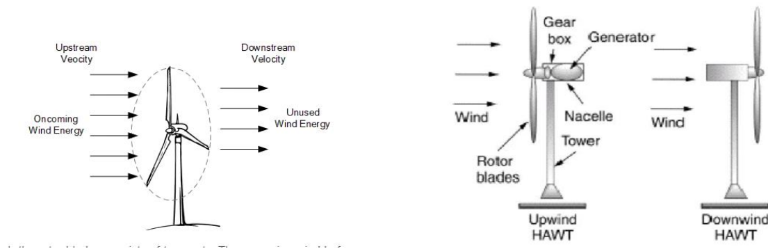
Figure 1: The horizontal axis wind turbine. (Francisco, 2019).
