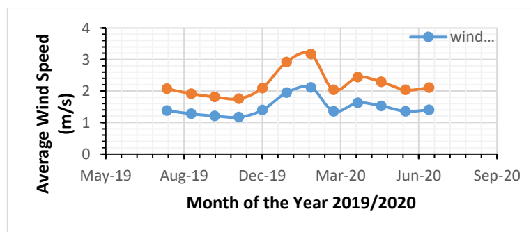
Figure 11. chart of average wind speed at different heights in 2019/2020
