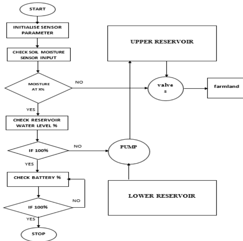
Figure 9 System Flowchart
