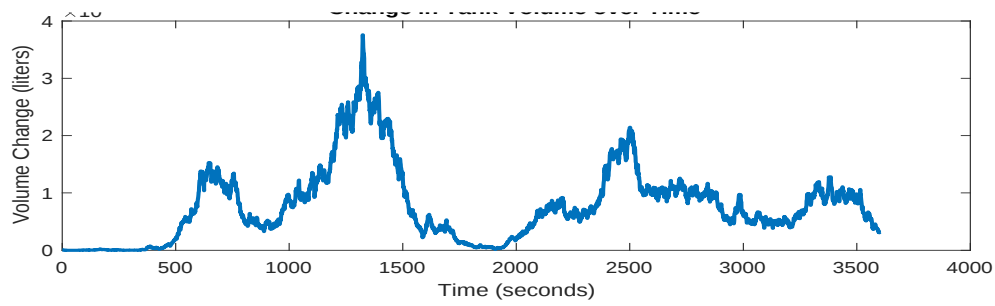
Figure. 20(a) Change in Reservoir Volume Over the Period of One Year
