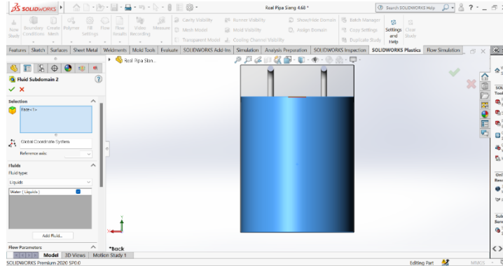
Figure 4. Input Fluid Subdomain of Water
