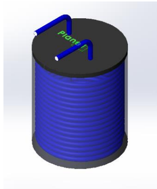
Figure 1. 3D Model of Heat Exchanger
