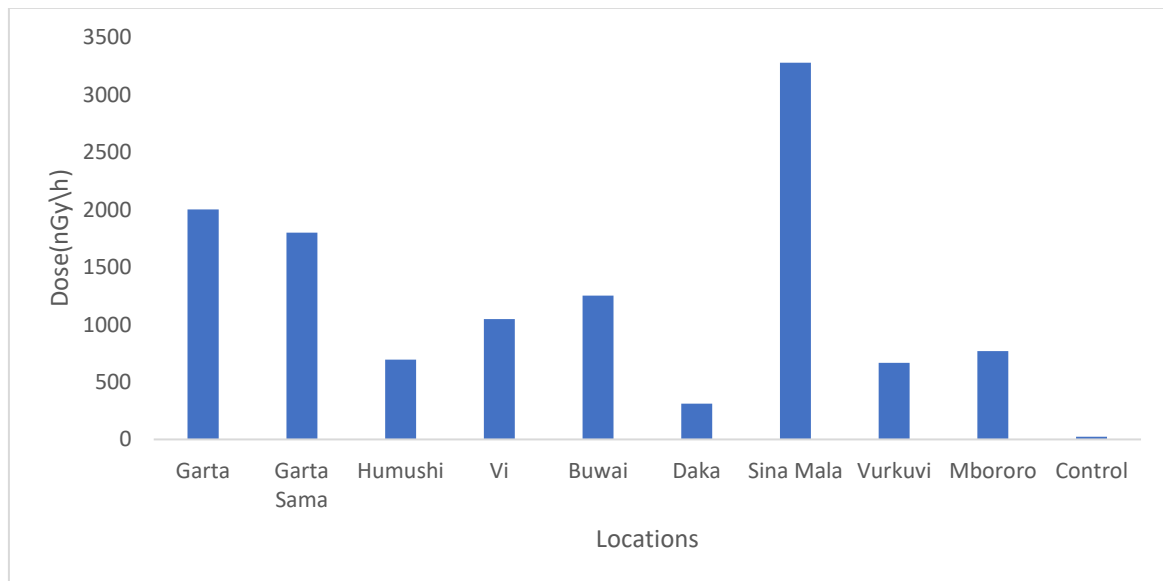
Figure 3: Absorbed Dose Rate of the soil sample
