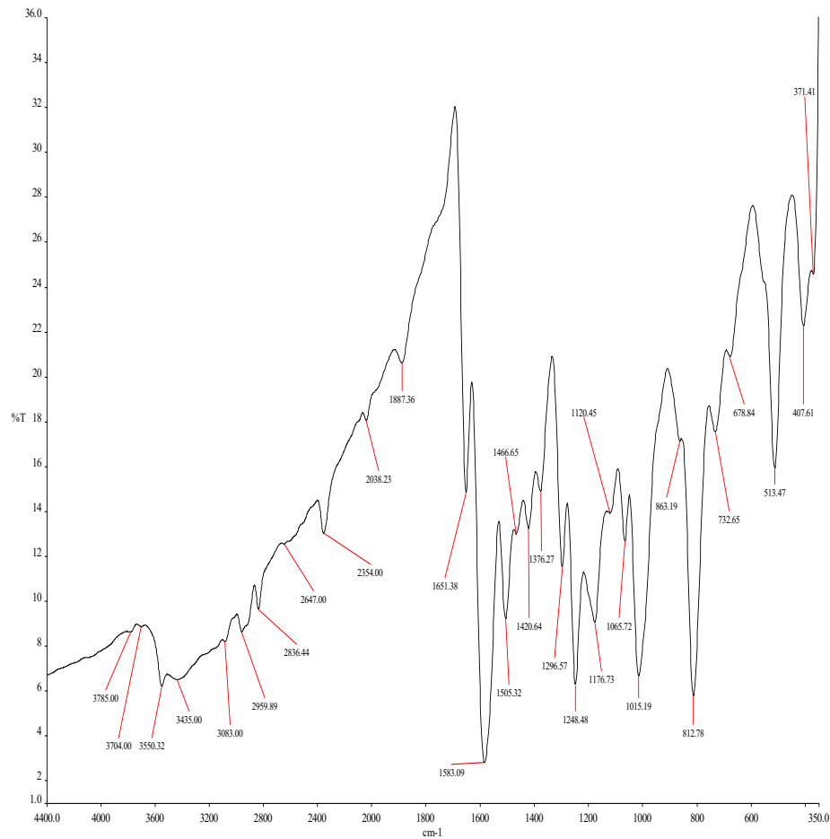
Figure 1. FTIR spectrum of Gongronema latifolium leaf extract
