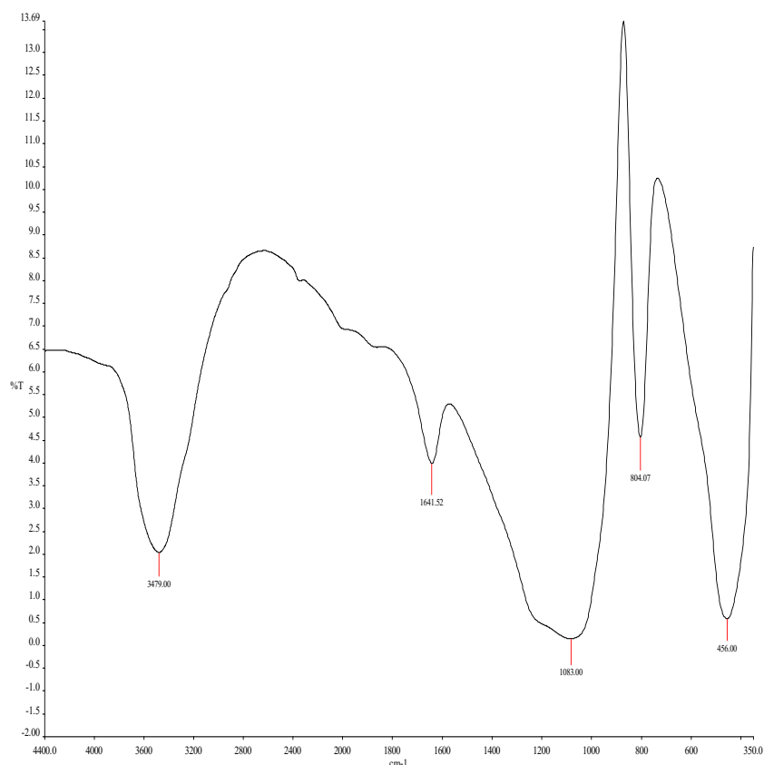
Figure 2. FTIR spectrum of Gongronema latifolium leaf hydrogel
