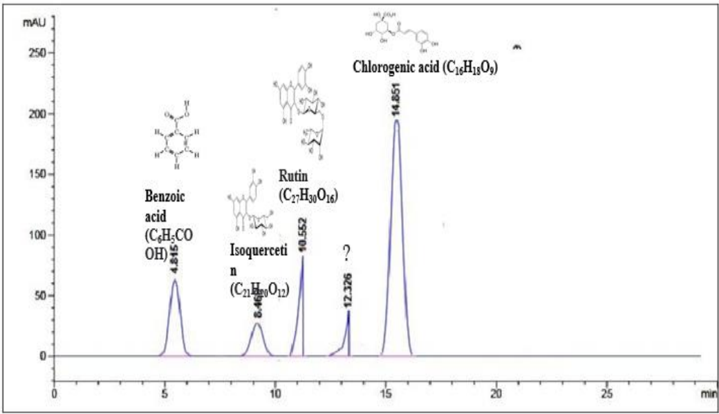
Figure 2: HPL chromatogram of flavonoids identified in aqueous bi-herbal root extract of Garcinia kola and Carica papaya (BH).
