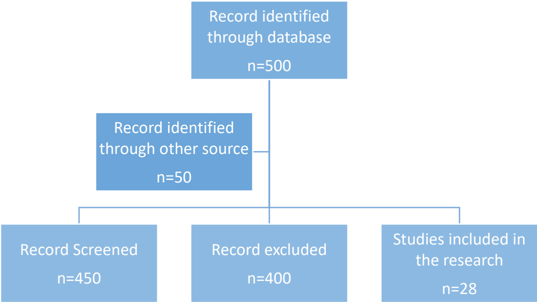
Figure 1. Prisma diagram
