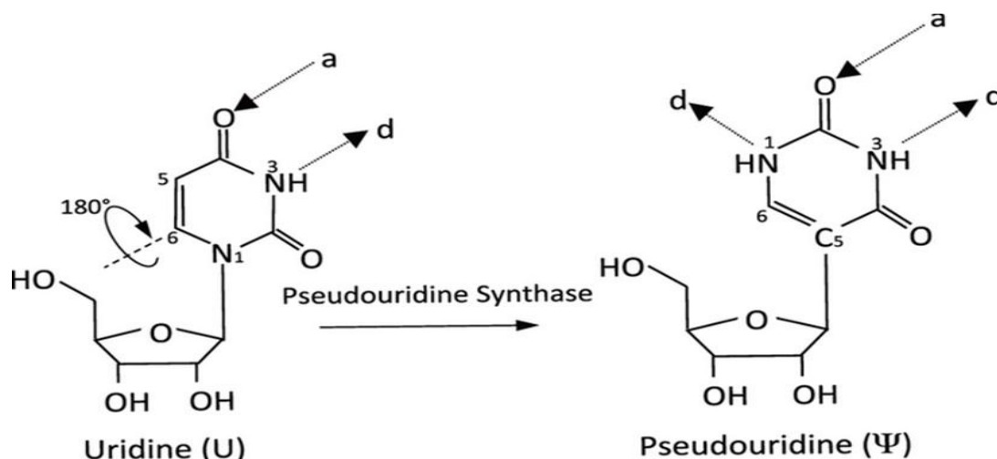
Figure 2: Schematic presentation of the Pseudouridation reaction: It results in an extra hydrogen bond donor (d) and the same number of hydrogen bond acceptors (a) (Zhao et al. , 2018).
