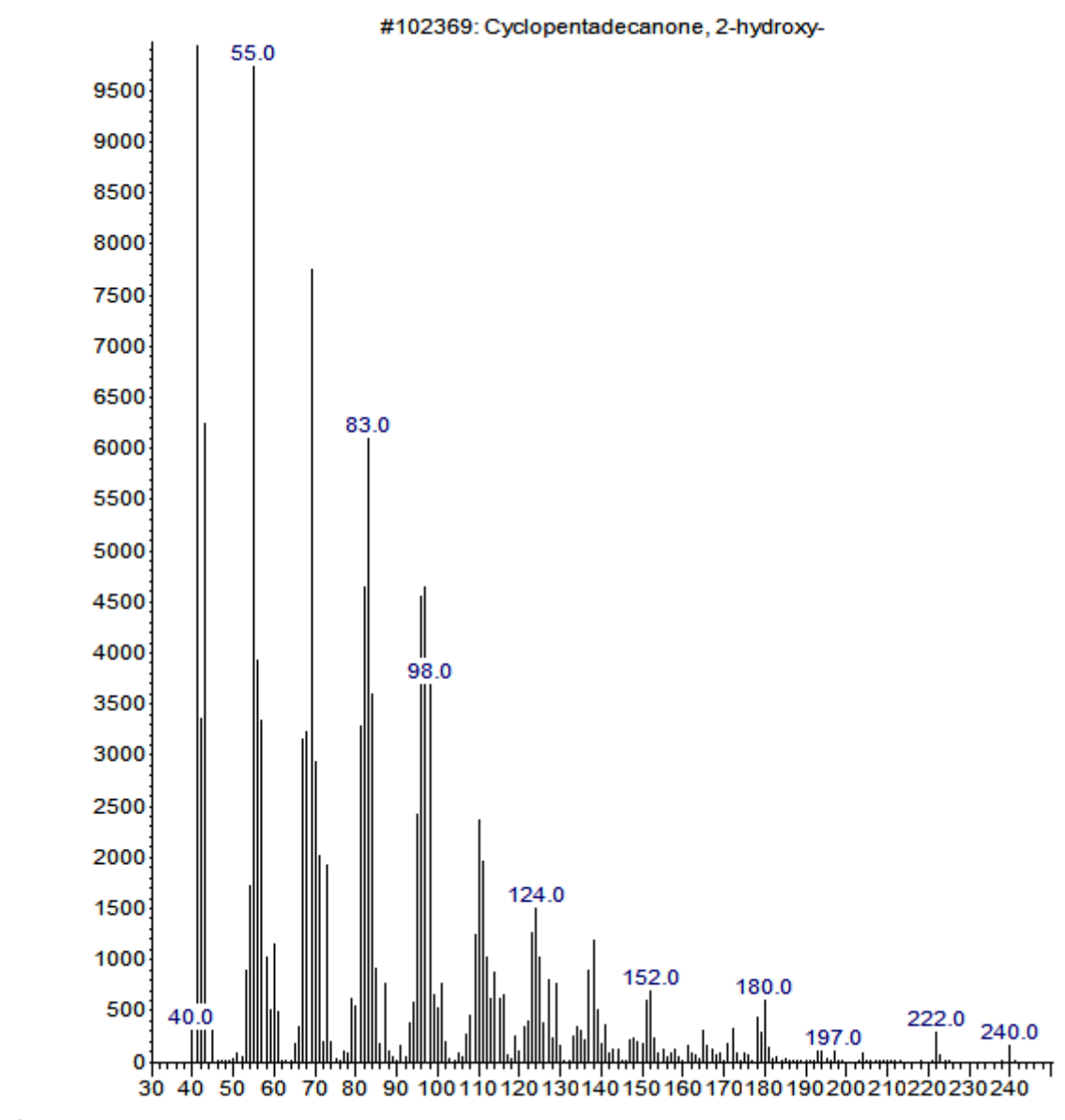
Figure 1. Peaks of GC-MS
