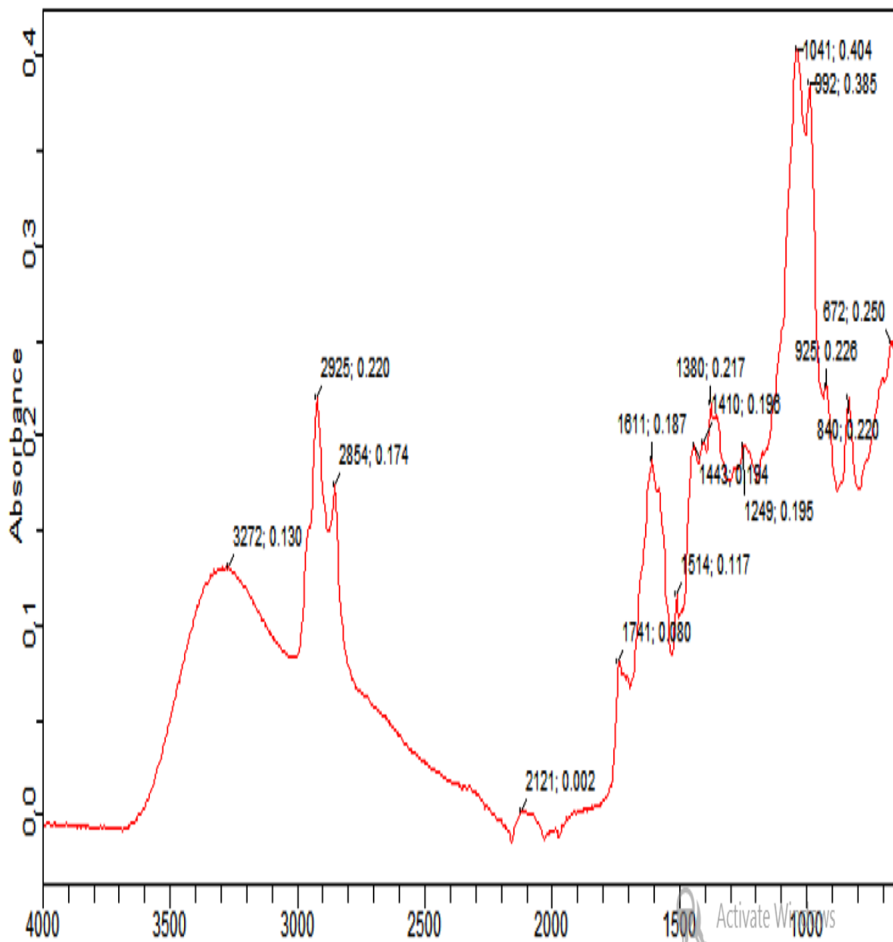
Figure 2: FTIR of the leaf extract.
