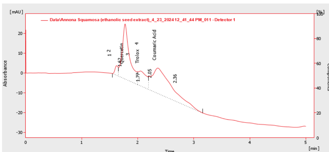
Figure 2. Chromatogram of the flavonoid profile of ethanol seed extract Annona squamosa
